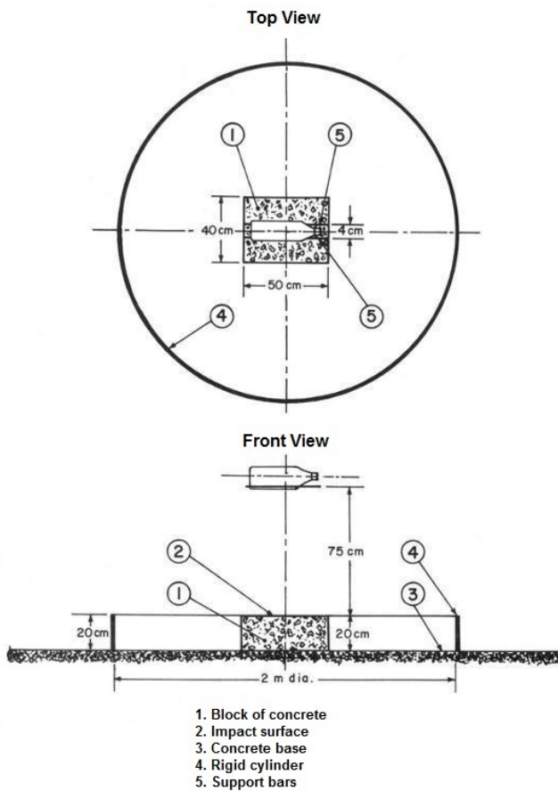
Figure — Test Apparatus
